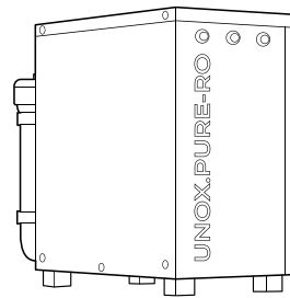
UNOX.PURE-RO reverse osmosis filtering system 230 x 540 x 445 mm - w x d x h Art. XHC002
