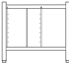
HIGH STAND for 600 x 400 COUNTERTOP ovens 842 x 713 x 752 mm - w x d x h Art.: XWARC-07EF-H
