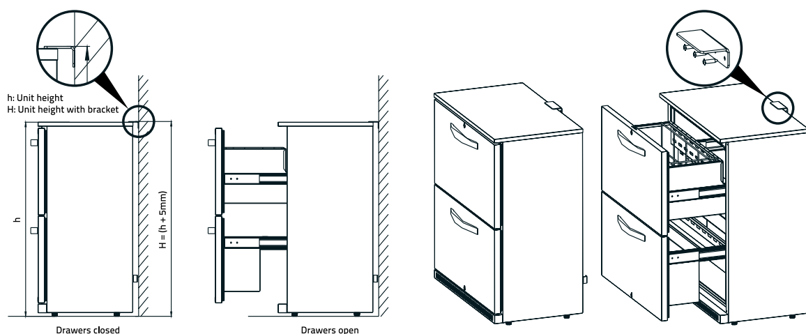
BRACKET INSTALLATION OPTION 1
