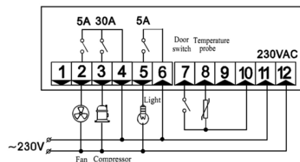
ELECTRONIC THERMOSTAT SF-402
