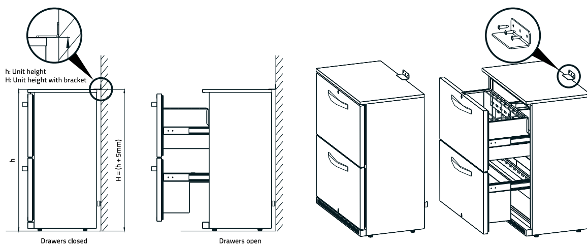
BRACKET INSTALLATION OPTION 2
